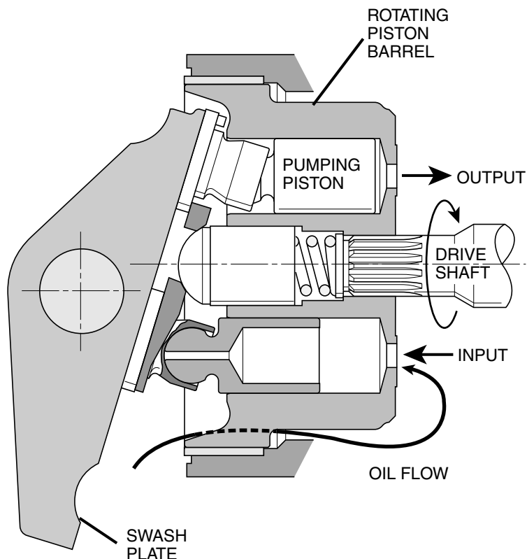
FIGURE 1. Pumping Action
